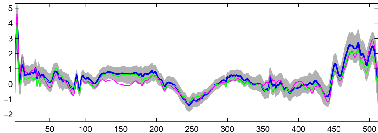
Estimated U_{28}(t) using R-WFMM: t_3 data, run 10
