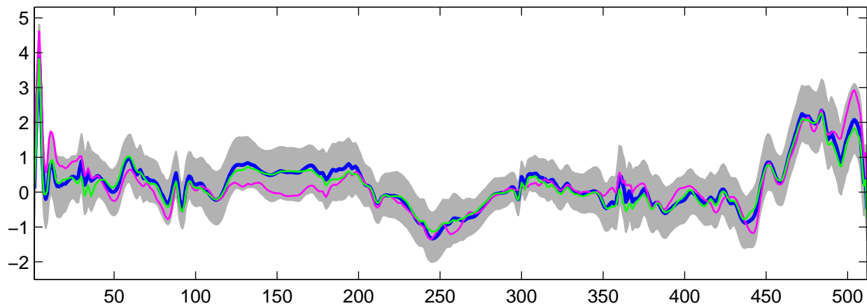
Estimated U_{28}(t) using G-WFMM: t_3 data, run 10
