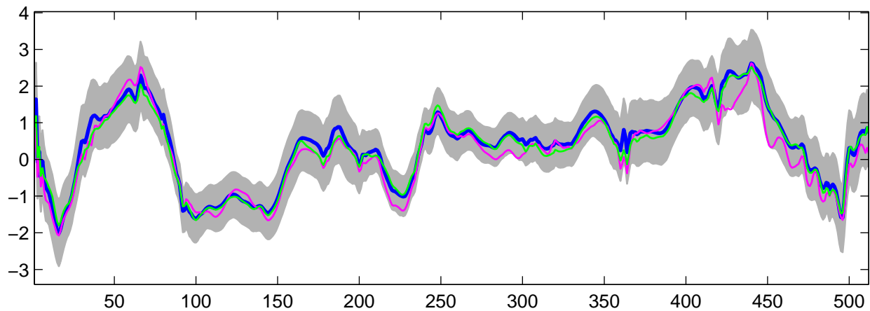
Estimated U_{29}(t) using G-WFMM: Normal data, run 10
