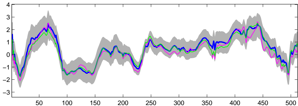
Estimated U_{29}(t) using R-WFMM: Normal data, run 10
