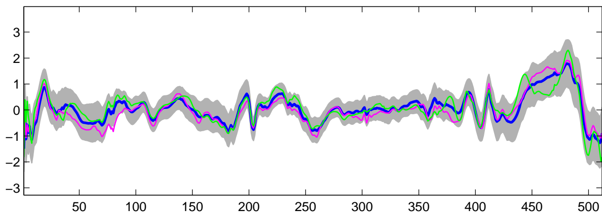
Estimated U_{29}(t) using R-WFMM: t_2 data, run 10
