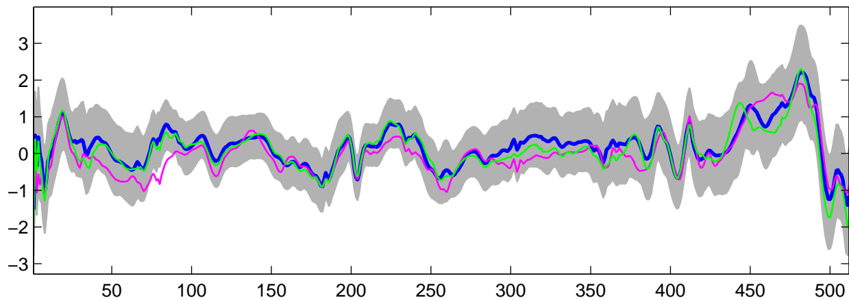
Estimated U_{29}(t) using G-WFMM: t_2 data, run 10
