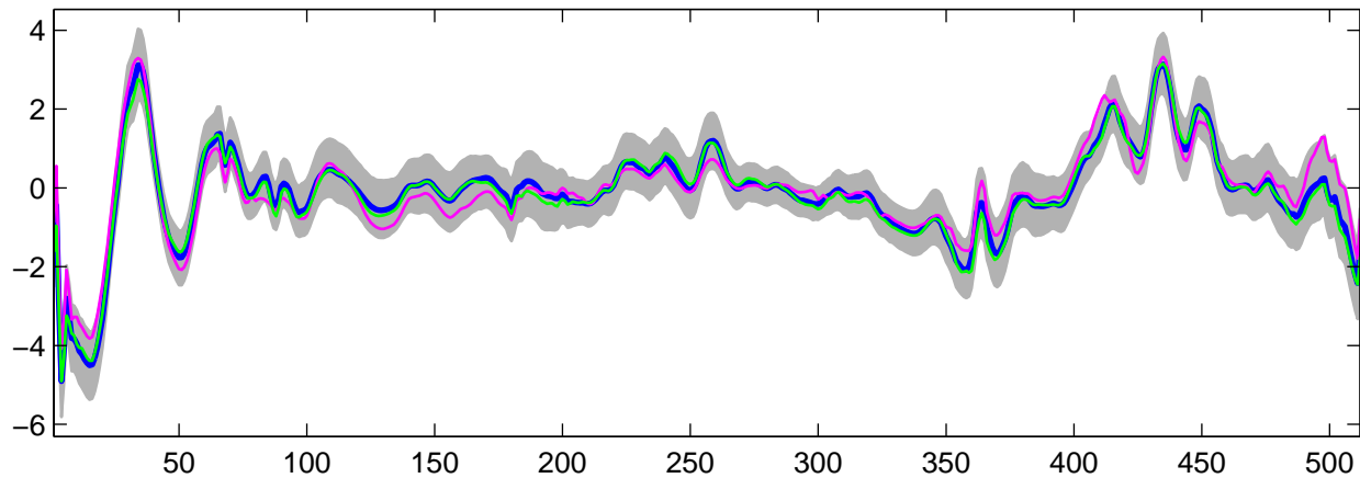
Estimated U_{29}(t) using G-WFMM: t_3 data, run 10
