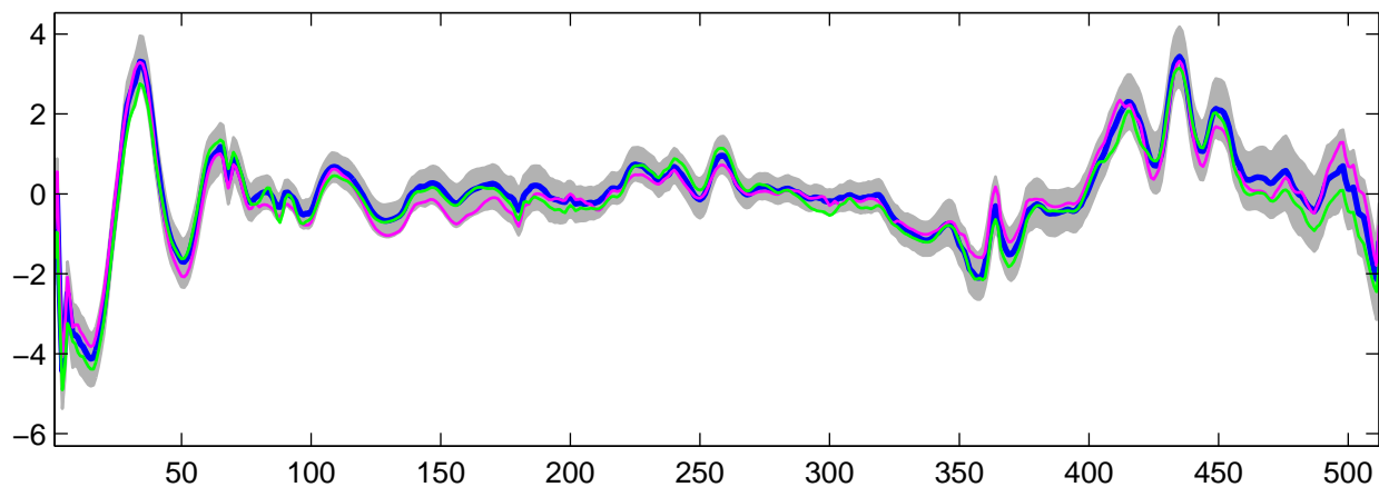
Estimated U_{29}(t) using R-WFMM: t_3 data, run 10
