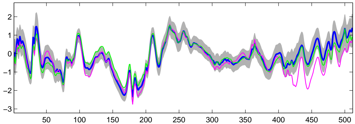
Estimated U_2(t) using R-WFMM: DE data, run 10
