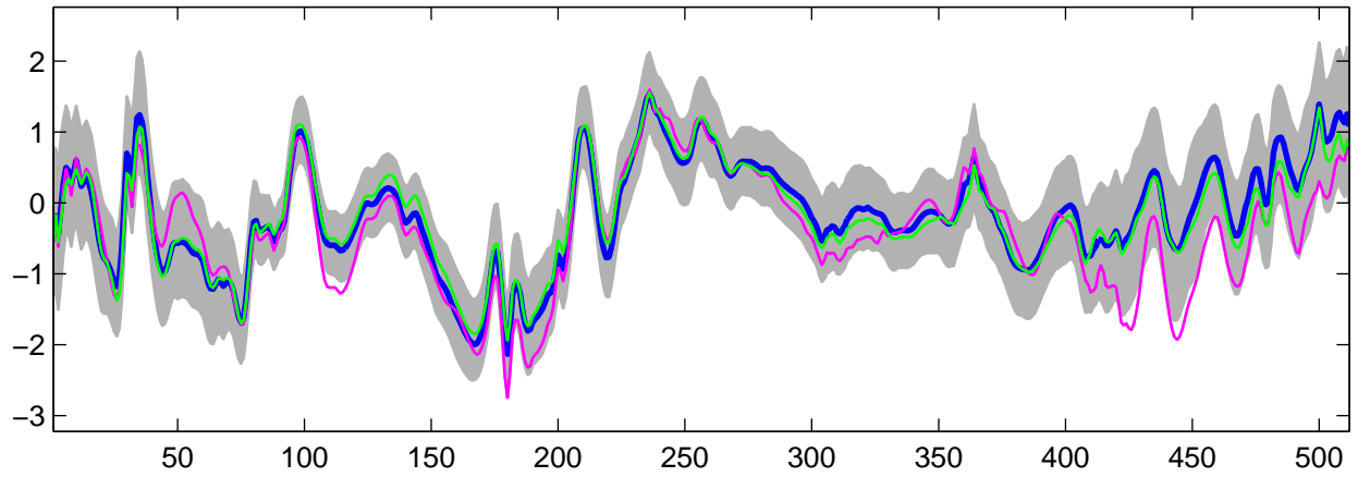
Estimated U_2(t) using G-WFMM: DE data, run 10
