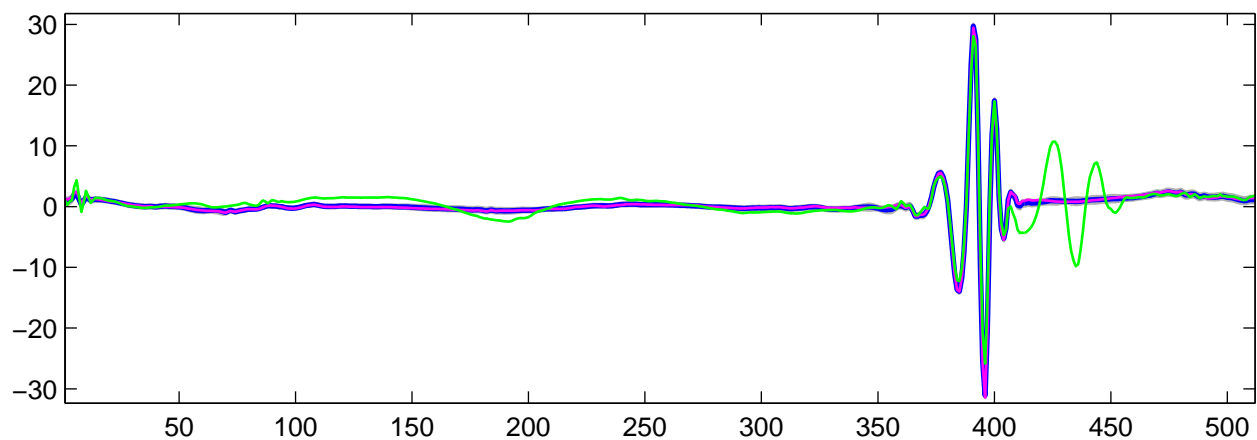
Estimated U_2(t) using R-WFMM: t_1 data, run 10
