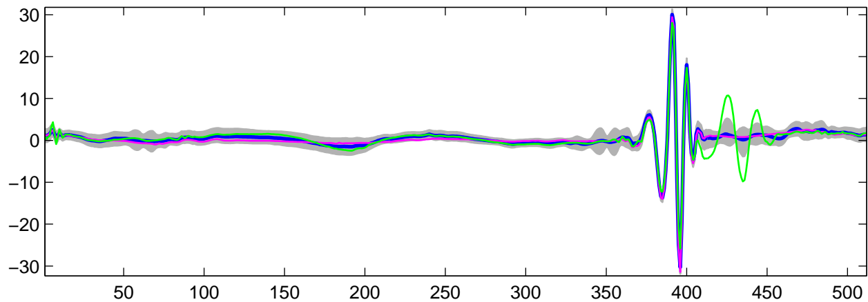
Estimated U_2(t) using G-WFMM: t_1 data, run 10
