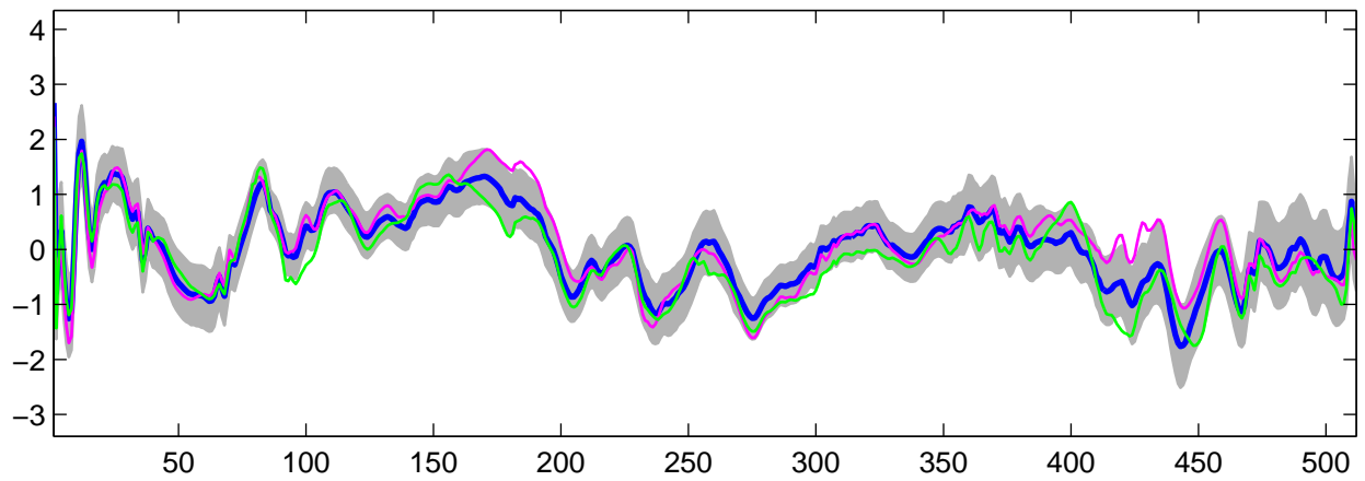
Estimated U_2(t) using R-WFMM: t_2 data, run 10
