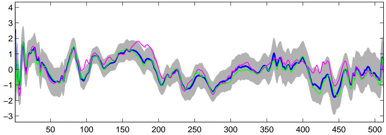
Estimated U_2(t) using G-WFMM: t_2 data, run 10
