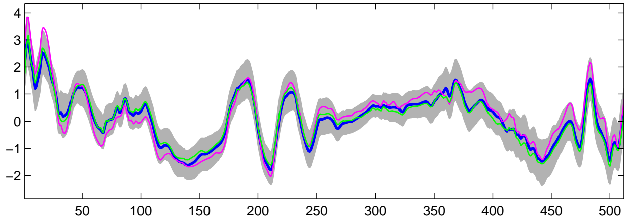
Estimated U_2(t) using G-WFMM: t_3 data, run 10
