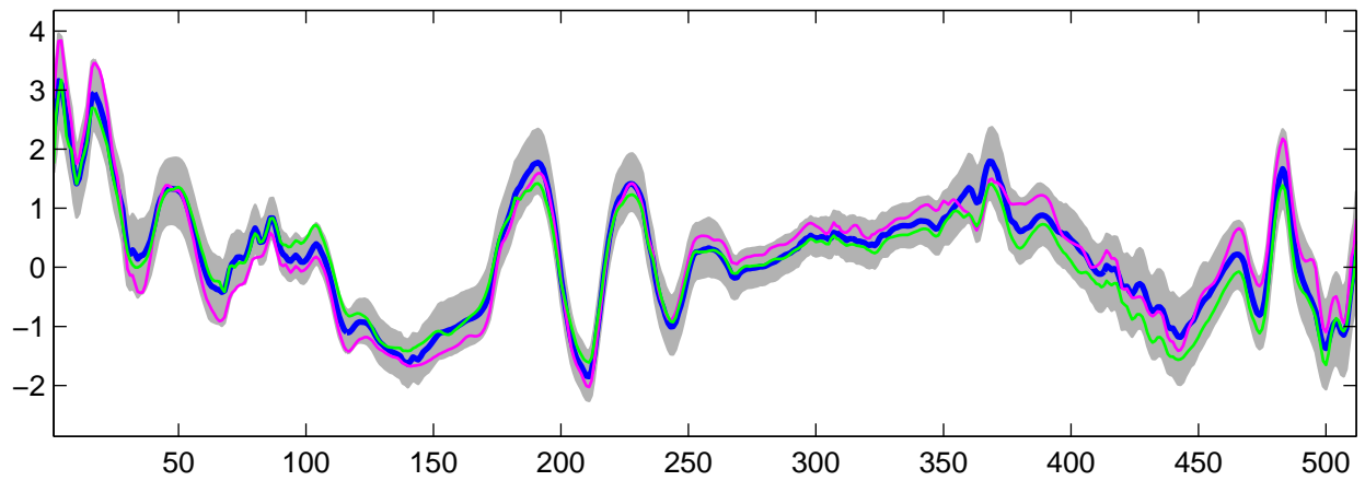
Estimated U_2(t) using R-WFMM: t_3 data, run 10
