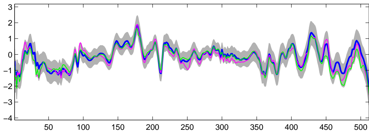
Estimated U_{30}(t) using R-WFMM: DE data, run 10
