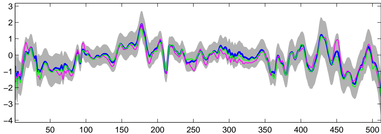
Estimated U_{30}(t) using G-WFMM: DE data, run 10
