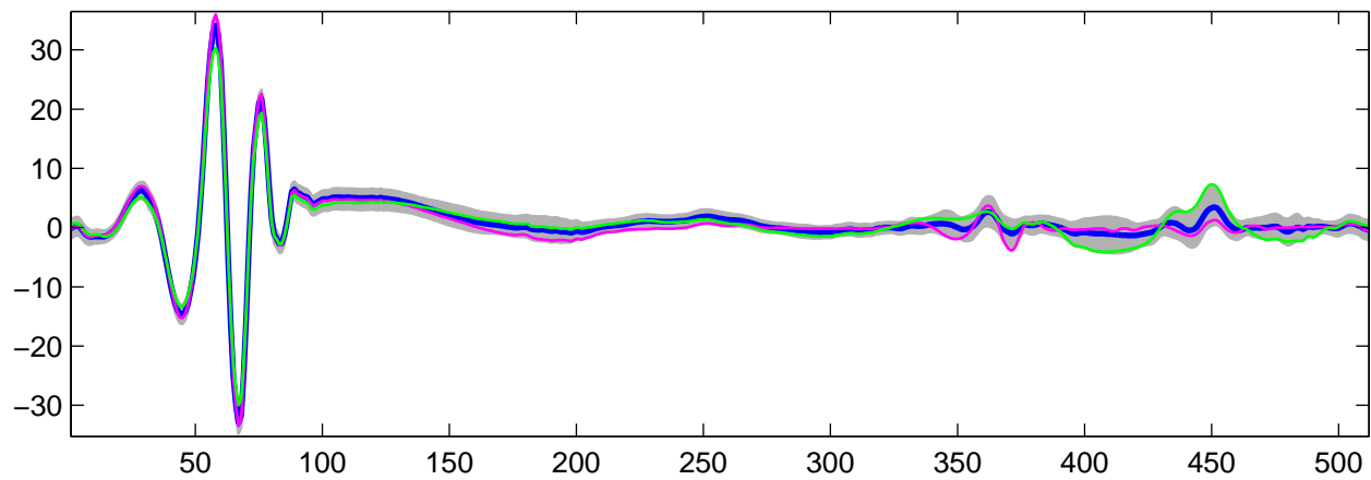
Estimated U_{30}(t) using G-WFMM: t_1 data, run 10
