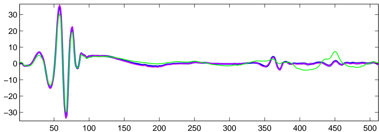
Estimated U_{30}(t) using R-WFMM: t_1 data, run 10
