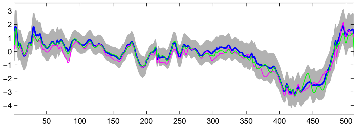
Estimated U_{30}(t) using G-WFMM: t_2 data, run 10
