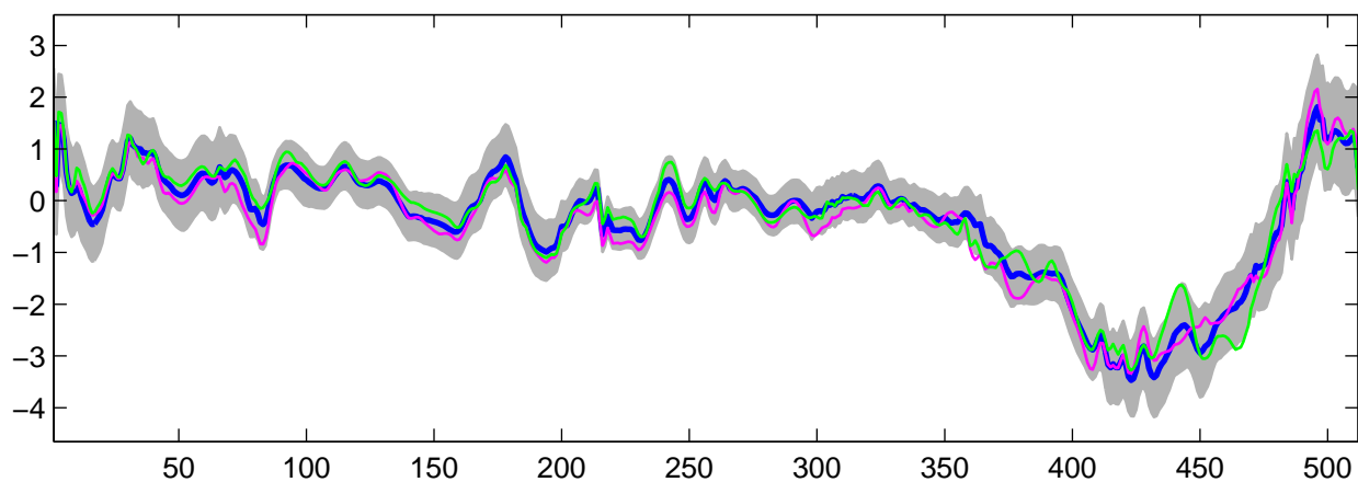
Estimated U_{30}(t) using R-WFMM: t_2 data, run 10
