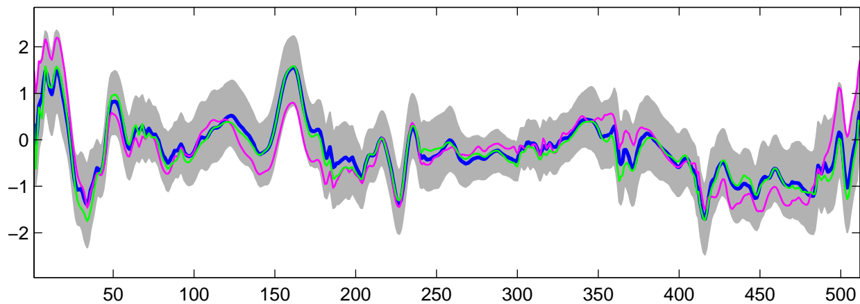
Estimated U_{30}(t) using G-WFMM: t_3 data, run 10
