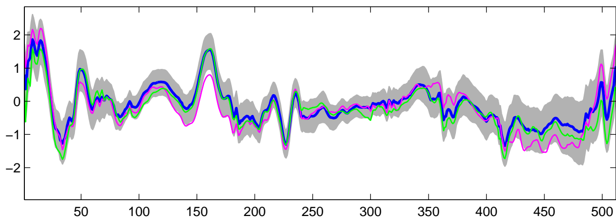
Estimated U_{30}(t) using R-WFMM: t_3 data, run 10
