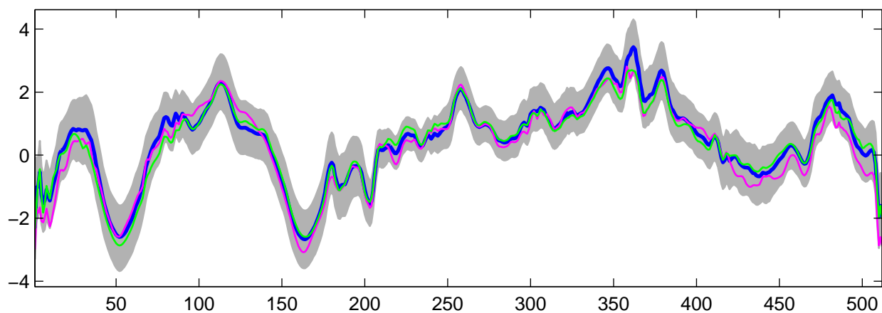
Estimated U_{31}(t) using R-WFMM: Normal data, run 10
