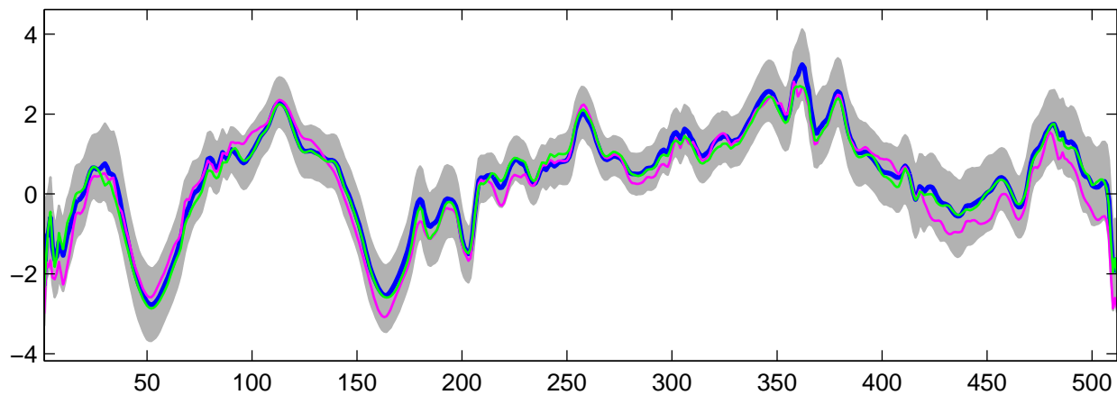
Estimated U_{31}(t) using G-WFMM: Normal data, run 10
