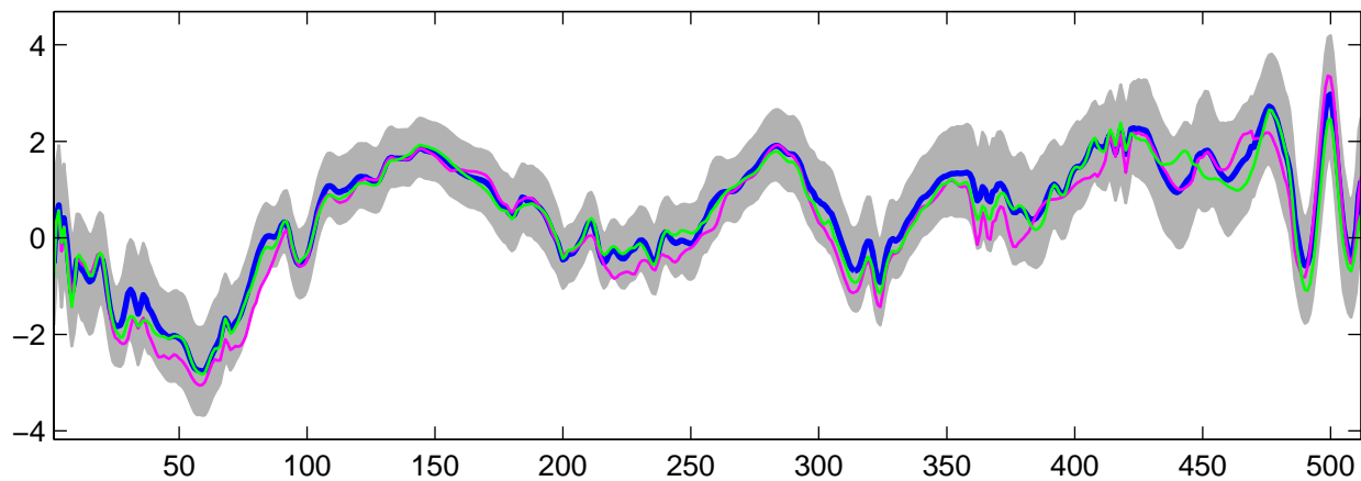
Estimated U_{31}(t) using G-WFMM: t_2 data, run 10
