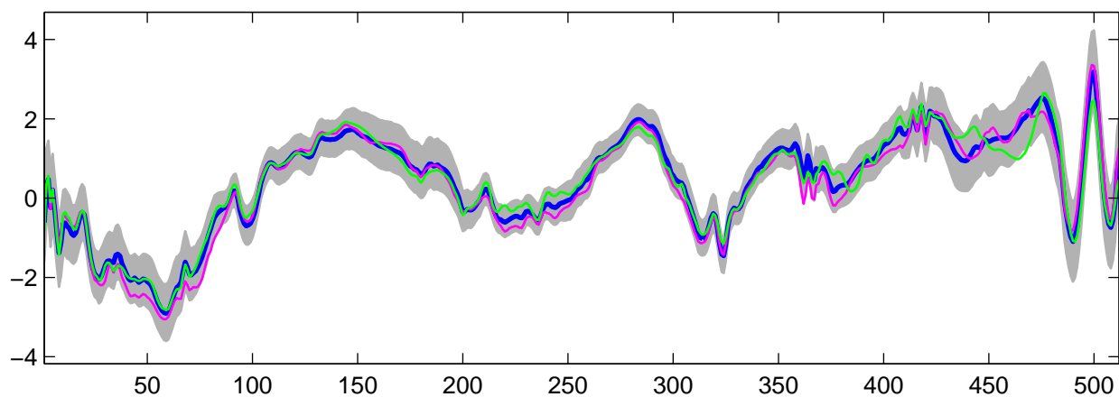
Estimated U_{31}(t) using R-WFMM: t_2 data, run 10
