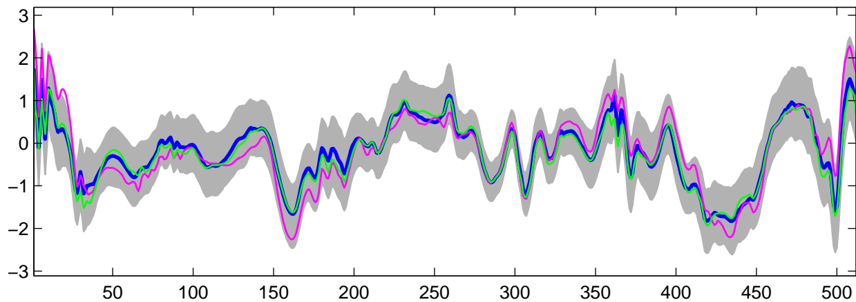
Estimated U_{31}(t) using G-WFMM: t_3 data, run 10
