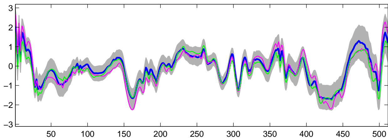
Estimated U_{31}(t) using R-WFMM: t_3 data, run 10
