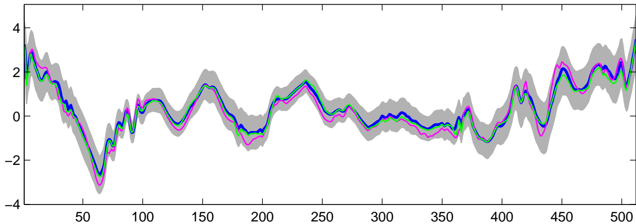
Estimated U_{32}(t) using G-WFMM: DE data, run 10
