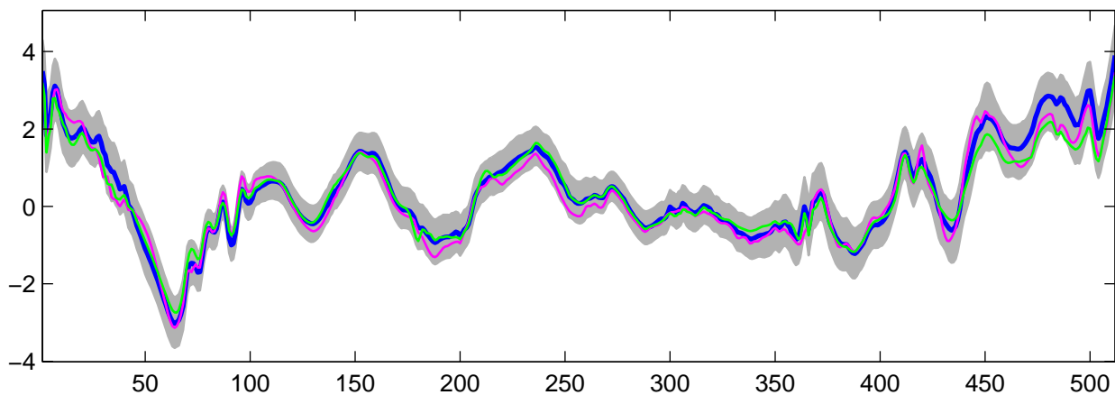
Estimated U_{32}(t) using R-WFMM: DE data, run 10
