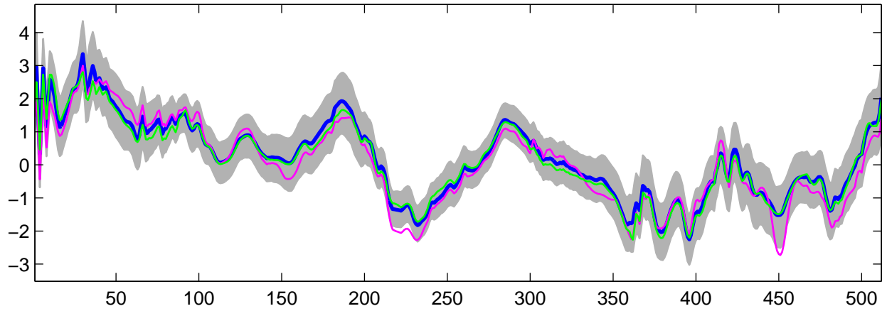
Estimated U_{32}(t) using G-WFMM: Normal data, run 10
