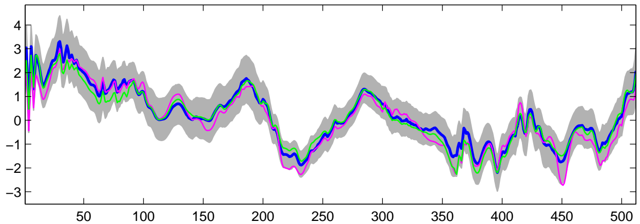
Estimated U_{32}(t) using R-WFMM: Normal data, run 10
