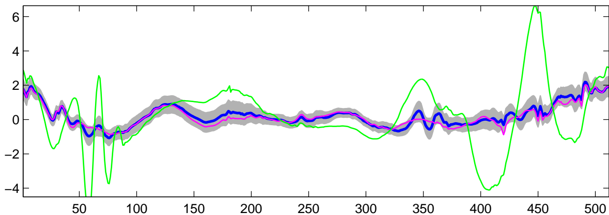
Estimated U_{32}(t) using R-WFMM: t_1 data, run 10
