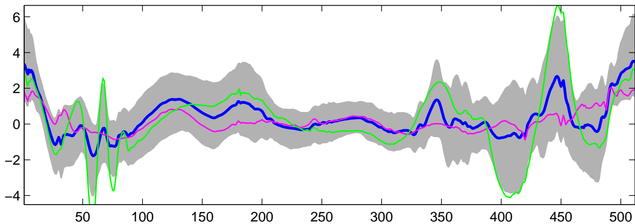
Estimated U_{32}(t) using G-WFMM: t_1 data, run 10
