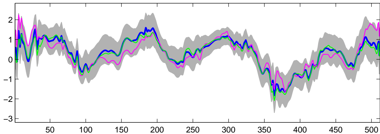
Estimated U_{32}(t) using G-WFMM: t_3 data, run 10
