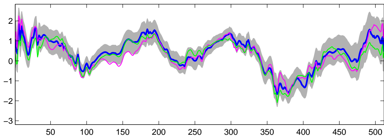
Estimated U_{32}(t) using R-WFMM: t_3 data, run 10
