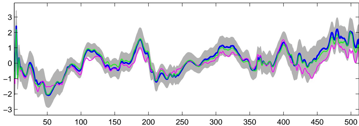
Estimated U_3(t) using G-WFMM: DE data, run 10
