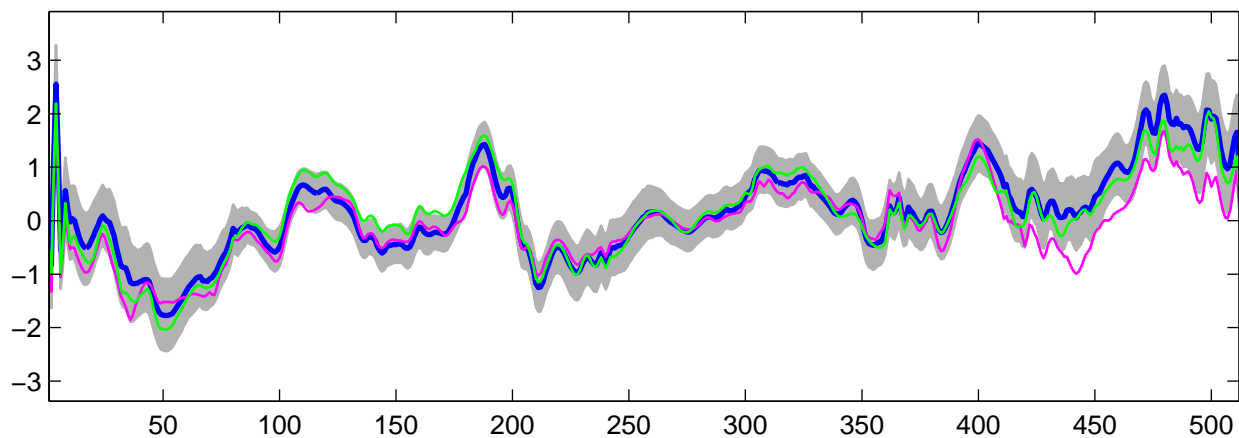
Estimated U_3(t) using R-WFMM: DE data, run 10
