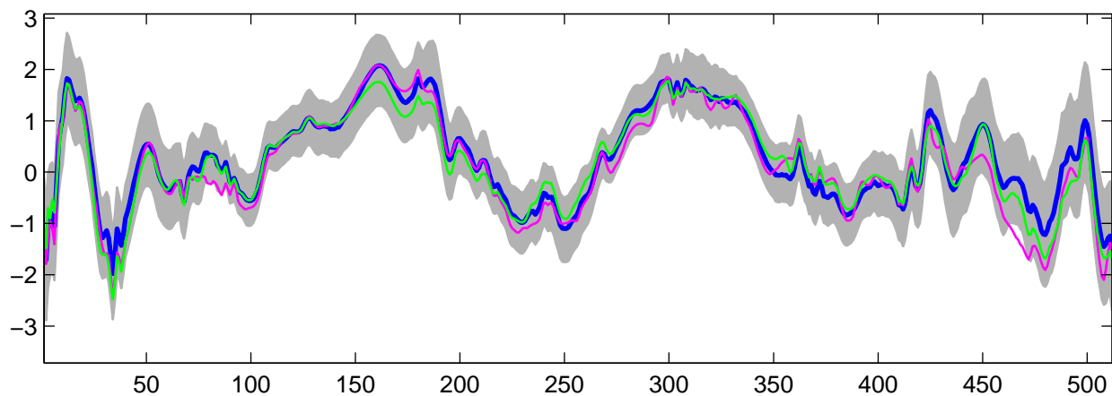
Estimated U_3(t) using R-WFMM: Normal data, run 10
