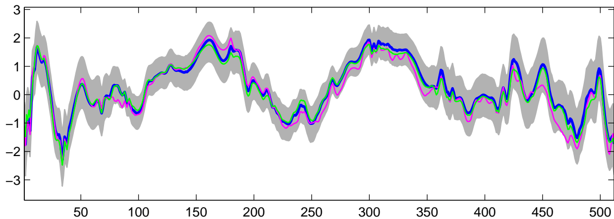
Estimated U_3(t) using G-WFMM: Normal data, run 10
