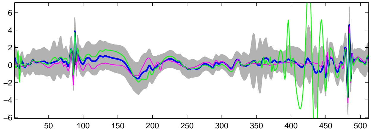
Estimated U_3(t) using G-WFMM: t_1 data, run 10
