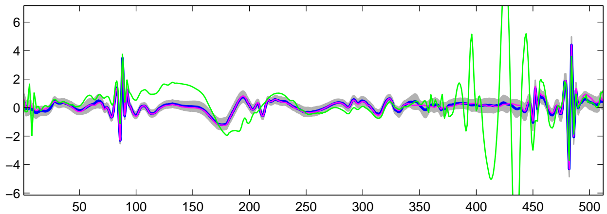
Estimated U_3(t) using R-WFMM: t_1 data, run 10
