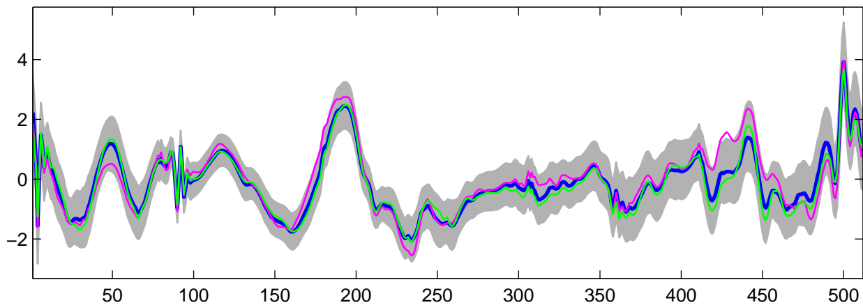
Estimated U_3(t) using G-WFMM: t_2 data, run 10
