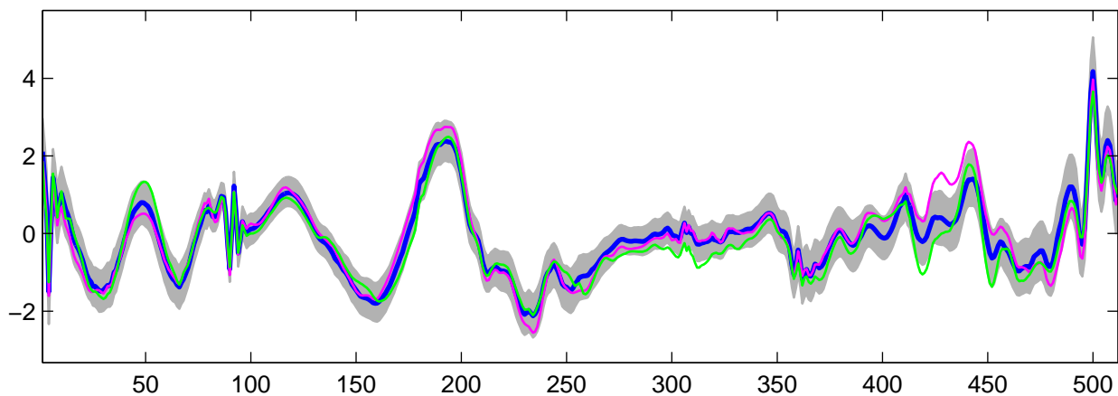
Estimated U_3(t) using R-WFMM: t_2 data, run 10
