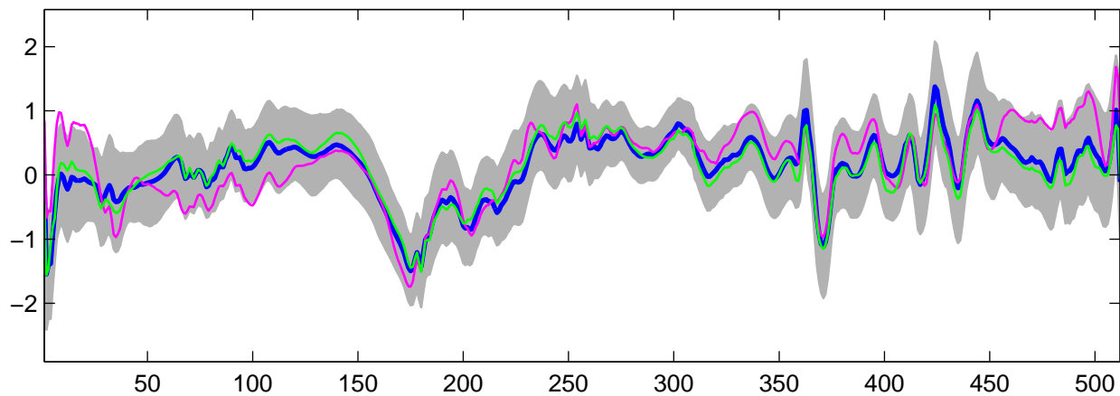
Estimated U_3(t) using G-WFMM: t_3 data, run 10
