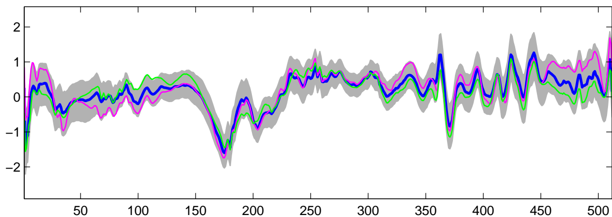
Estimated U_3(t) using R-WFMM: t_3 data, run 10
