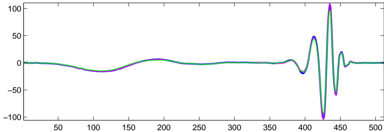
Estimated U_4(t) using R-WFMM: t_1 data, run 10
