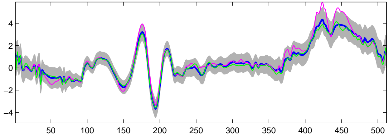
Estimated U_4(t) using G-WFMM: t_2 data, run 10
