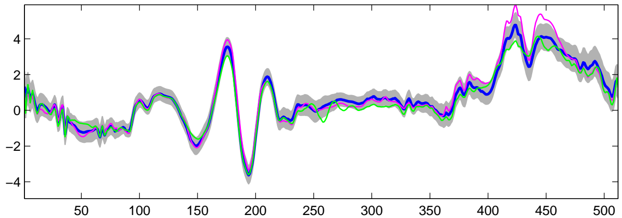
Estimated U_4(t) using R-WFMM: t_2 data, run 10
