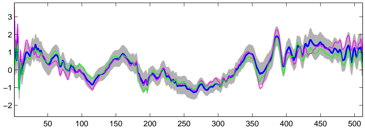
Estimated U_4(t) using R-WFMM: t_3 data, run 10
