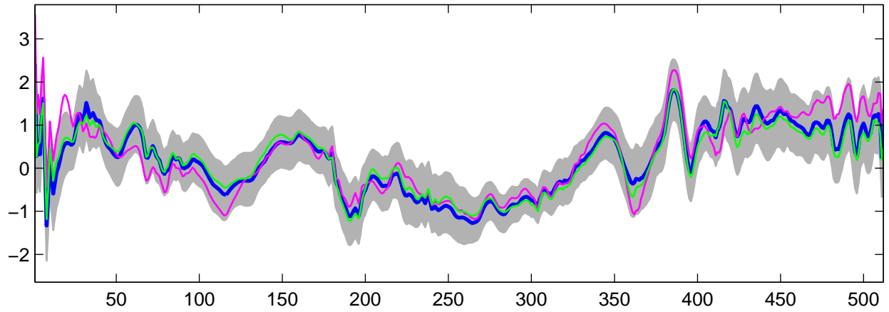
Estimated U_4(t) using G-WFMM: t_3 data, run 10
