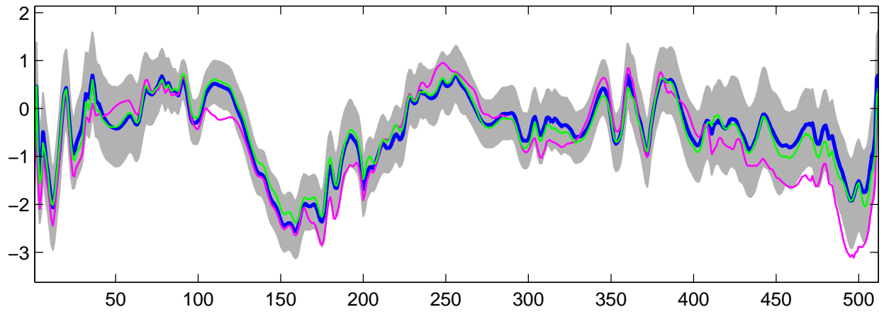
Estimated U_5(t) using G-WFMM: DE data, run 10
