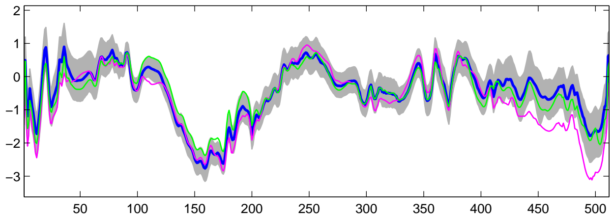
Estimated U_5(t) using R-WFMM: DE data, run 10
