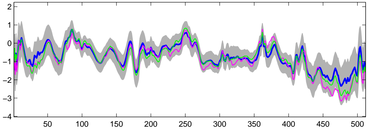
Estimated U_5(t) using R-WFMM: Normal data, run 10
