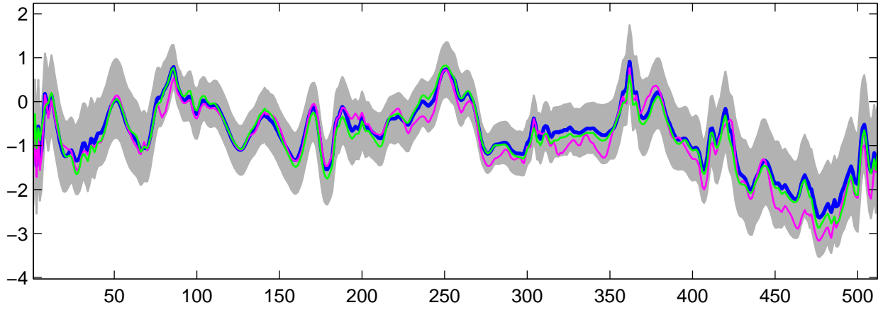
Estimated U_5(t) using G-WFMM: Normal data, run 10
