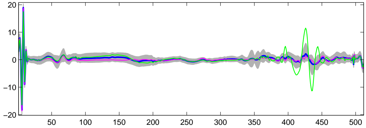
Estimated U_5(t) using G-WFMM: t_1 data, run 10
