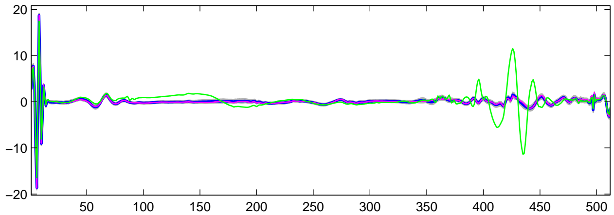
Estimated U_5(t) using R-WFMM: t_1 data, run 10
