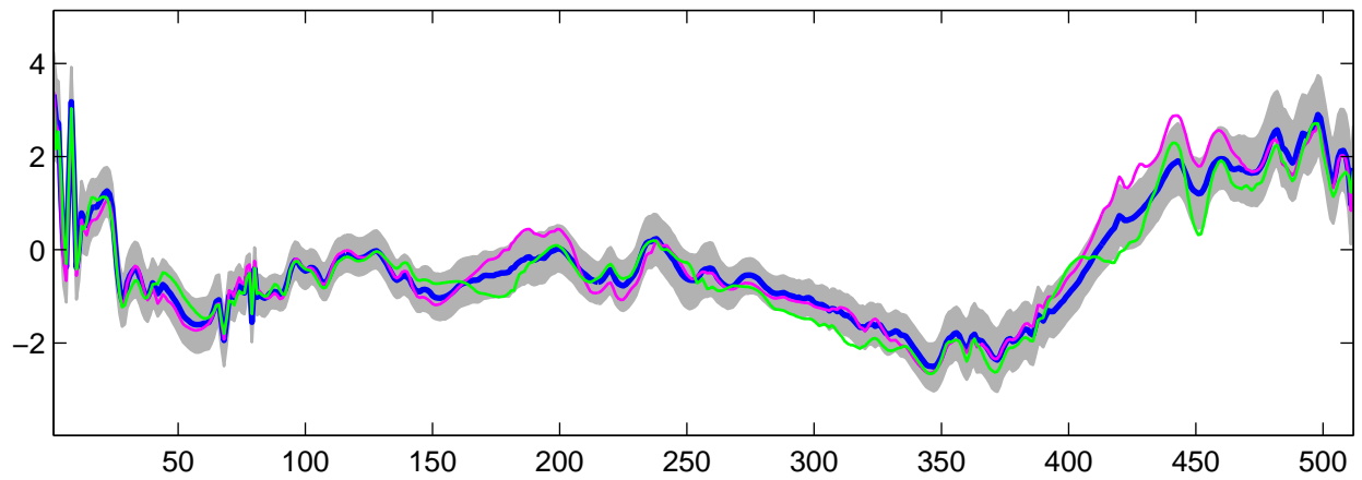
Estimated U_5(t) using R-WFMM: t_2 data, run 10
