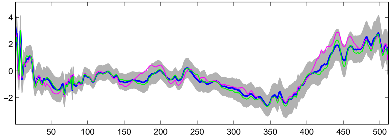
Estimated U_5(t) using G-WFMM: t_2 data, run 10
