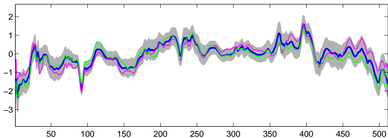
Estimated U_5(t) using R-WFMM: t_3 data, run 10
