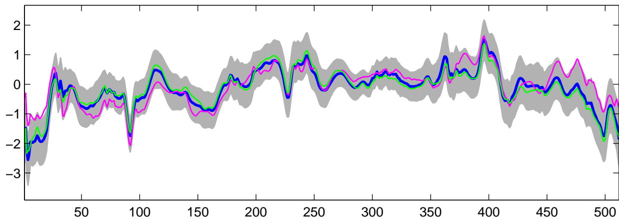
Estimated U_5(t) using G-WFMM: t_3 data, run 10
