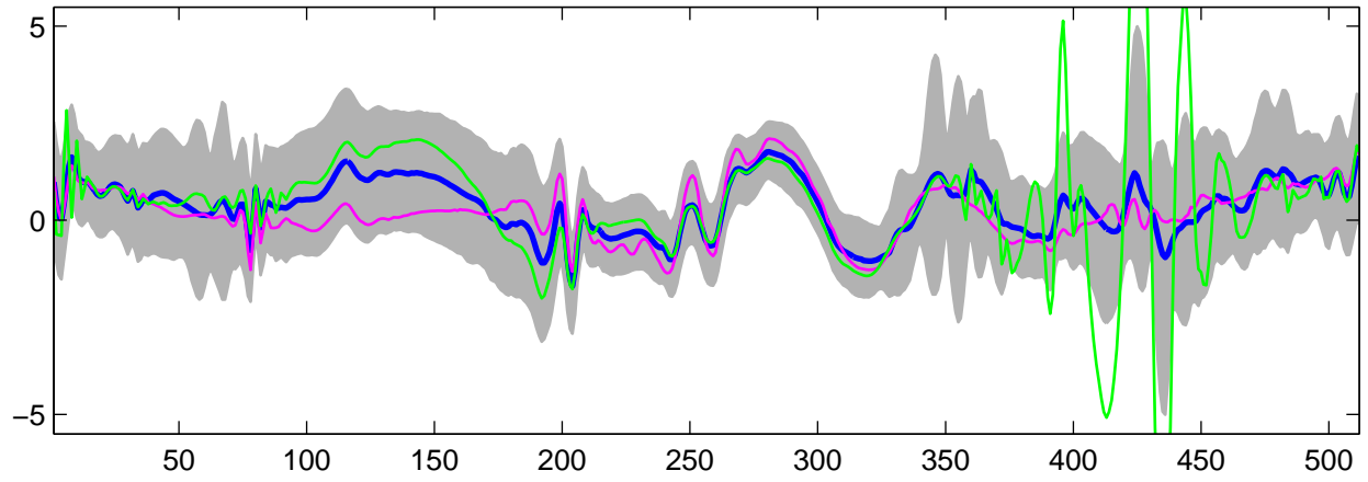
Estimated U_6(t) using G-WFMM: t_1 data, run 10
