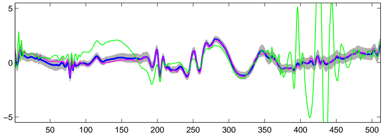
Estimated U_6(t) using R-WFMM: t_1 data, run 10
