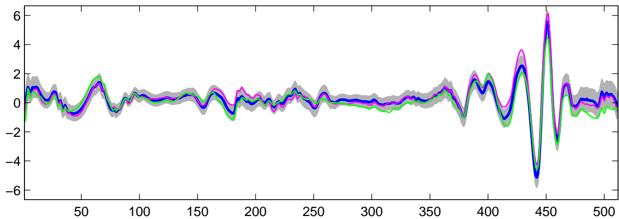
Estimated U_6(t) using R-WFMM: t_2 data, run 10
