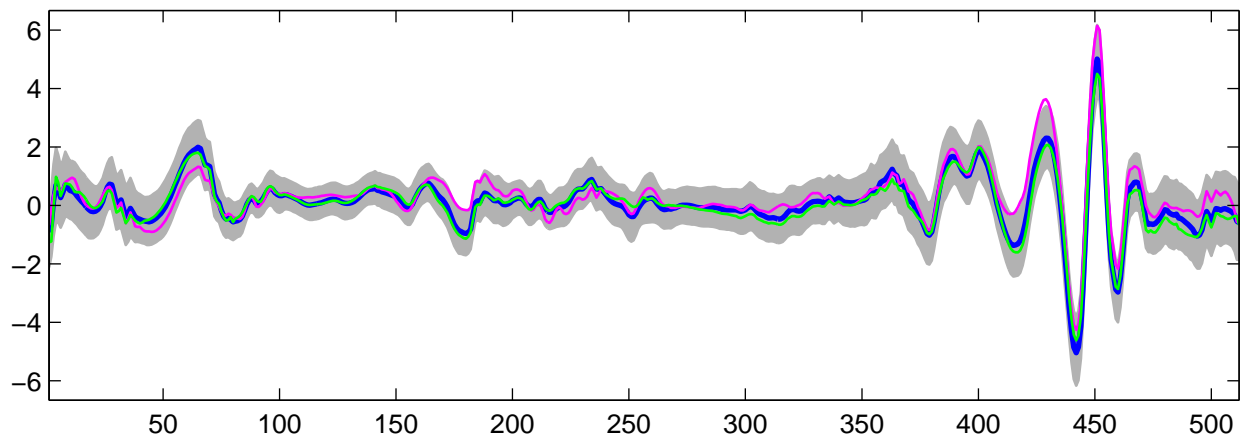
Estimated U_6(t) using G-WFMM: t_2 data, run 10
