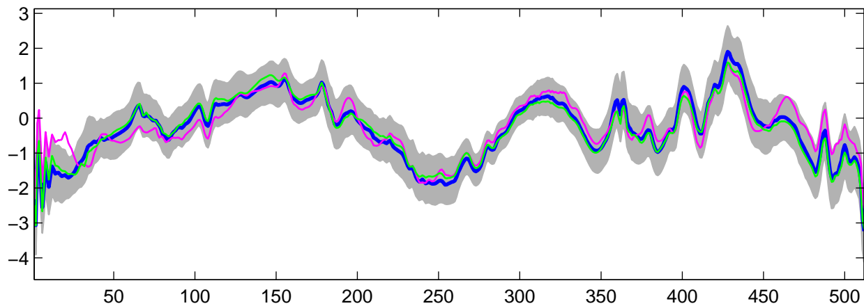
Estimated U_6(t) using G-WFMM: t_3 data, run 10
