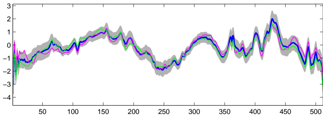
Estimated U_6(t) using R-WFMM: t_3 data, run 10
