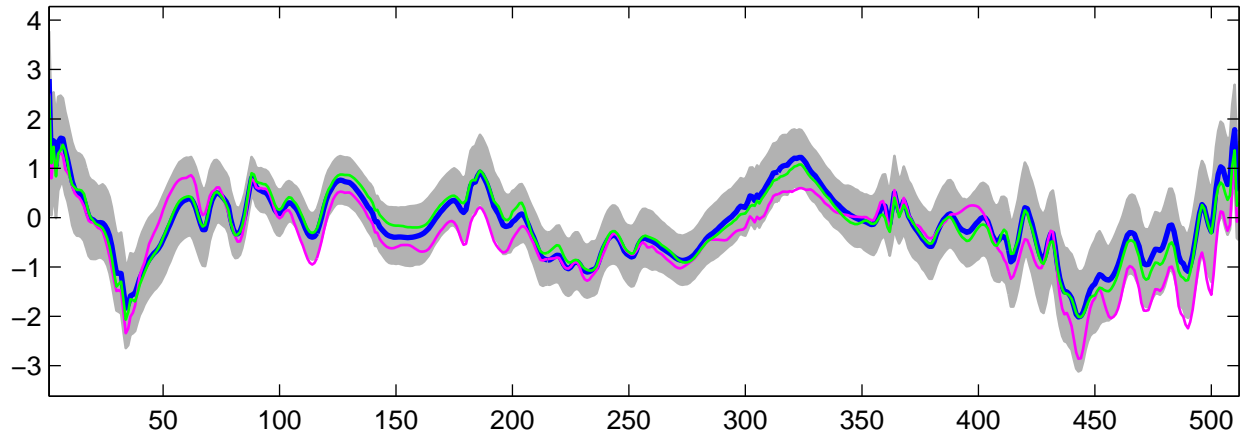
Estimated U_7(t) using G-WFMM: DE data, run 10
