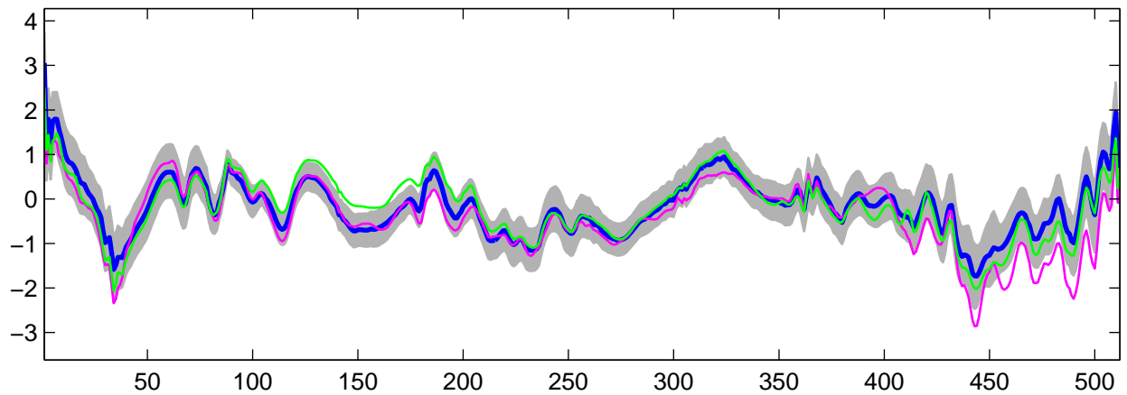
Estimated U_7(t) using R-WFMM: DE data, run 10
