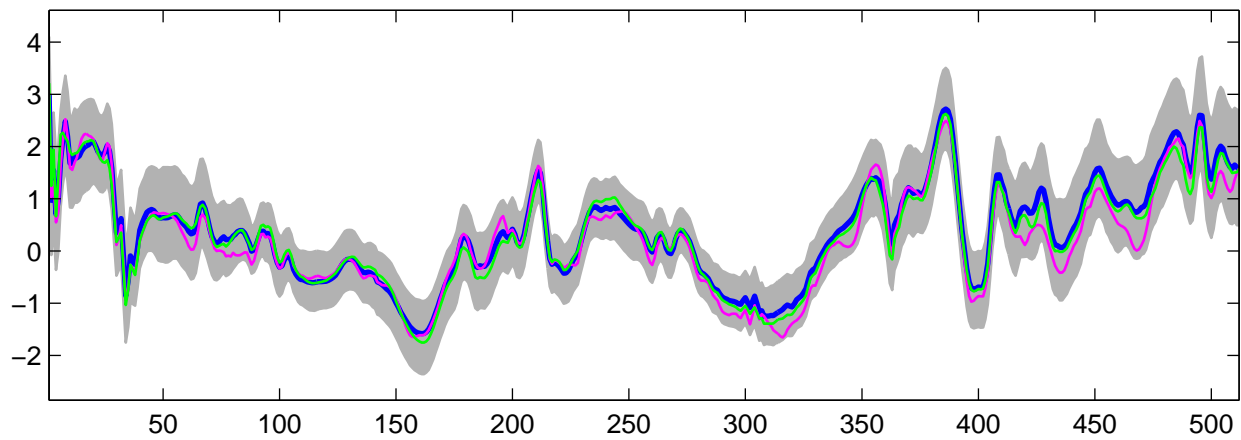
Estimated U_7(t) using G-WFMM: Normal data, run 10
