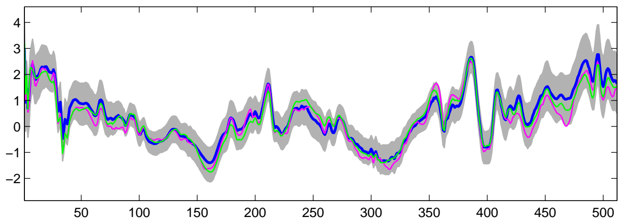
Estimated U_7(t) using R-WFMM: Normal data, run 10
