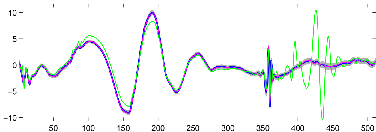
Estimated U_7(t) using R-WFMM: t_1 data, run 10
