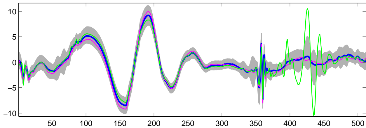
Estimated U_7(t) using G-WFMM: t_1 data, run 10
