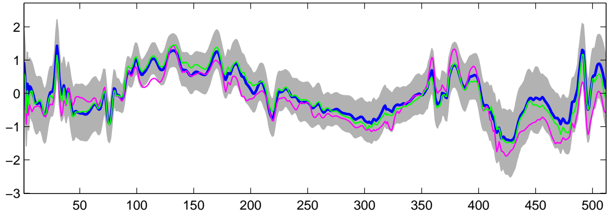
Estimated U_g(t) using G-WFMM: DE data, run 10
