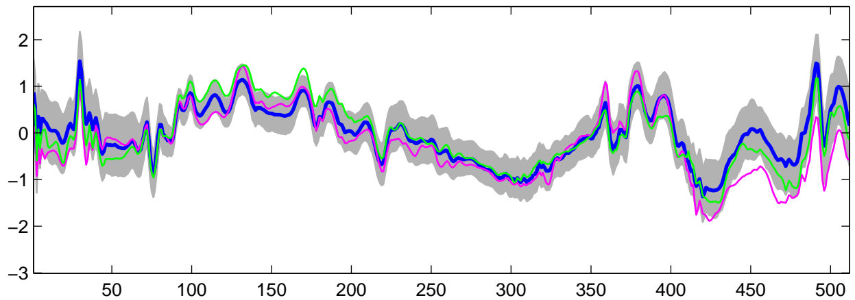
Estimated U_g(t) using R-WFMM: DE data, run 10
