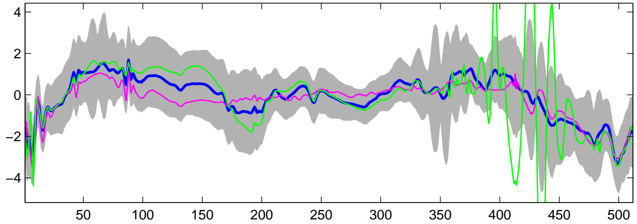
Estimated U_g(t) using G-WFMM: t_1 data, run 10
