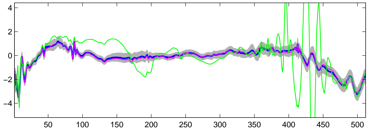
Estimated U_g(t) using R-WFMM: t_1 data, run 10
