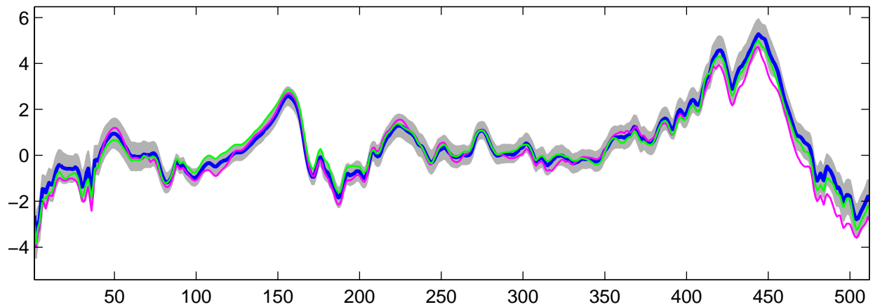
Estimated U_{\theta}(t) using R-WFMM: DE data, run 10
