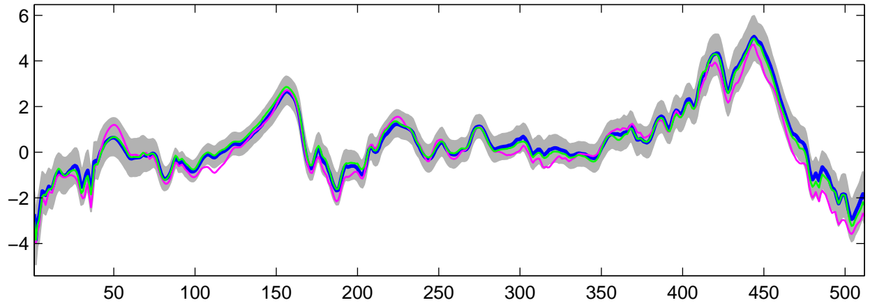
Estimated U_{\theta}(t) using G-WFMM: DE data, run 10
