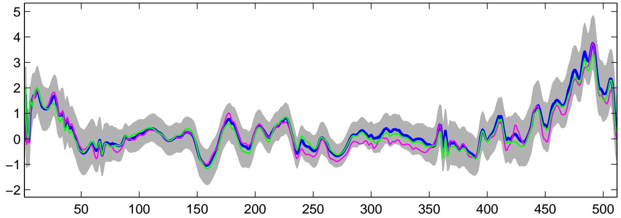
Estimated U_{\theta}(t) using G-WFMM: Normal data, run 10
