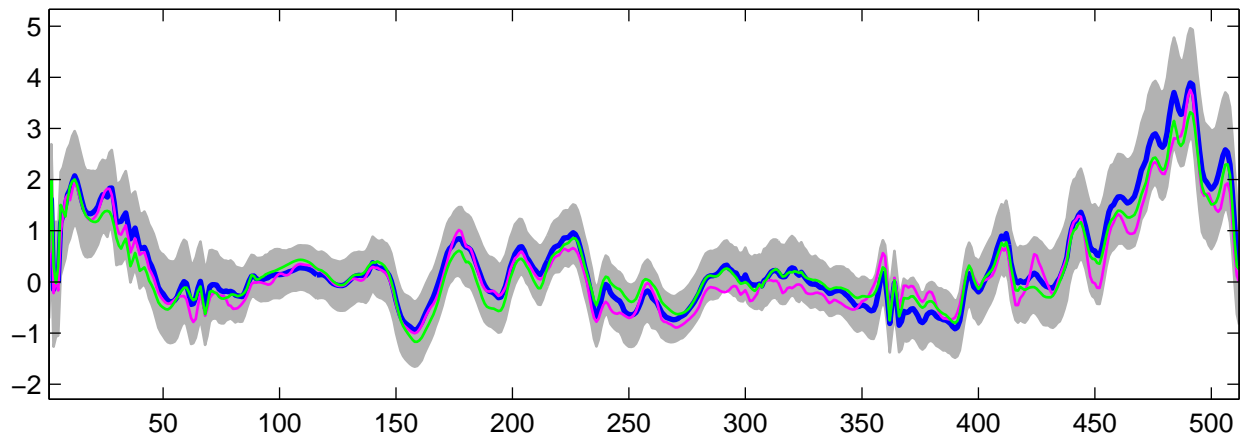
Estimated U_{\theta}(t) using R-WFMM: Normal data, run 10
