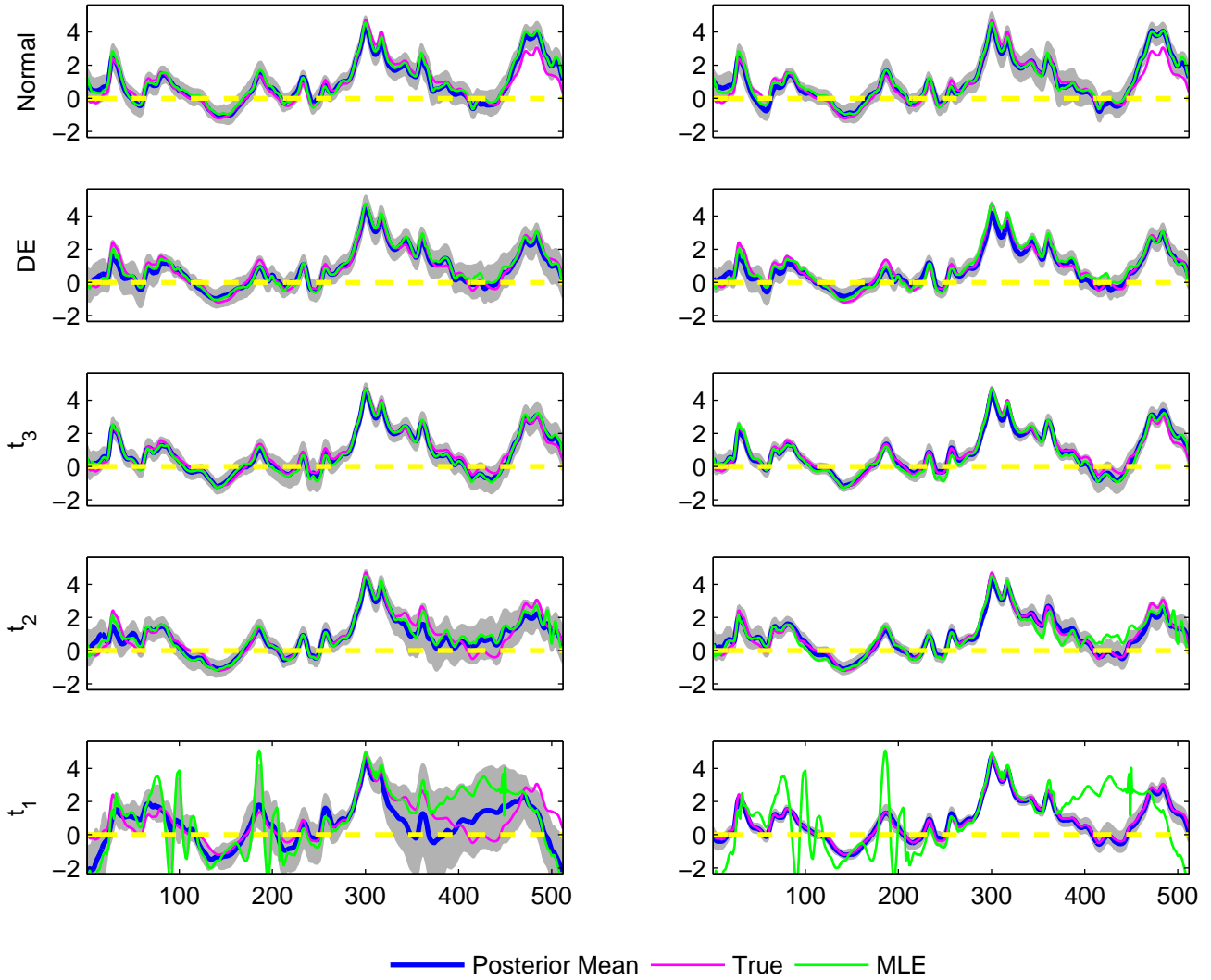
The estimated B_1(t) for 5 simulated datasets, simulation run 2 G-WFMM R-WFMM
