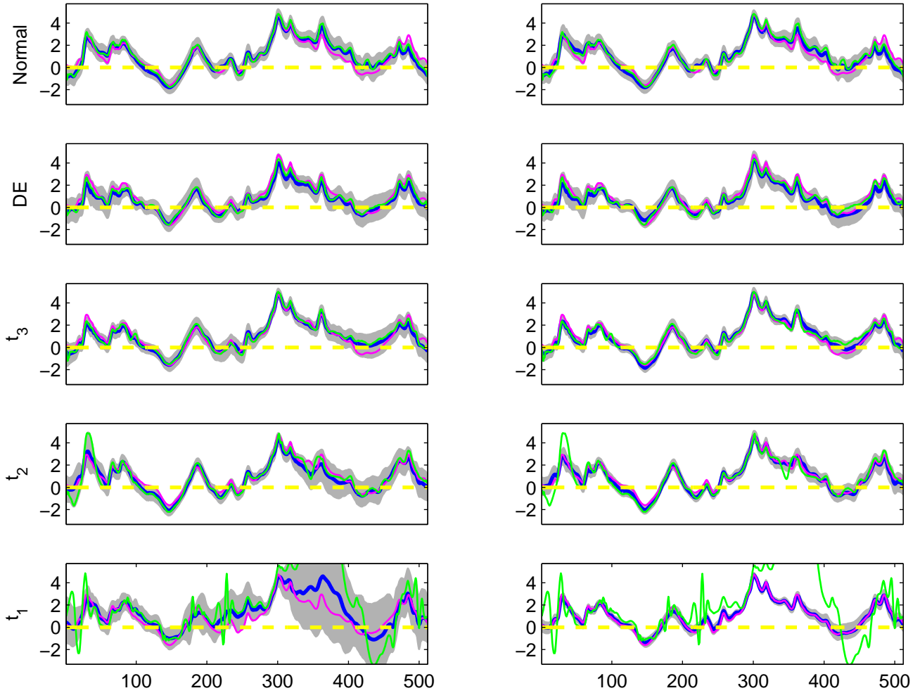
The estimated B_2(t) for 5 simulated datasets, simulation run 2 G-WFMM R-WFMM
