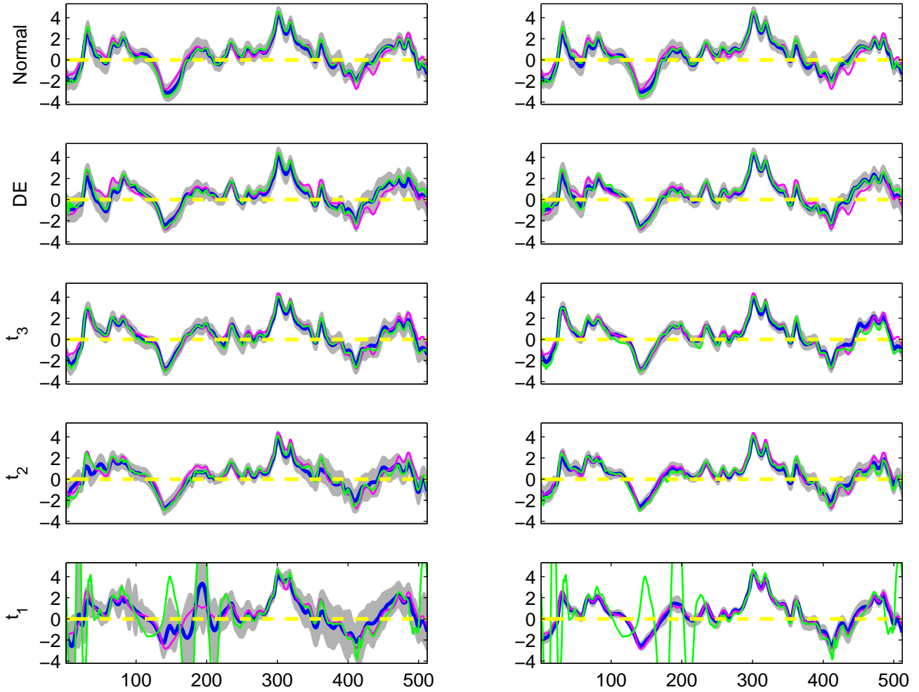
The estimated B_3(t) for 5 simulated datasets, simulation run 2 G-WFMM R-WFMM
