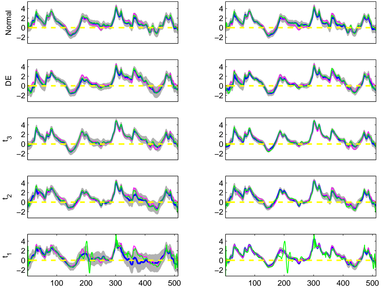
The estimated B_4(t) for 5 simulated datasets, simulation run 2 G-WFMM R-WFMM
