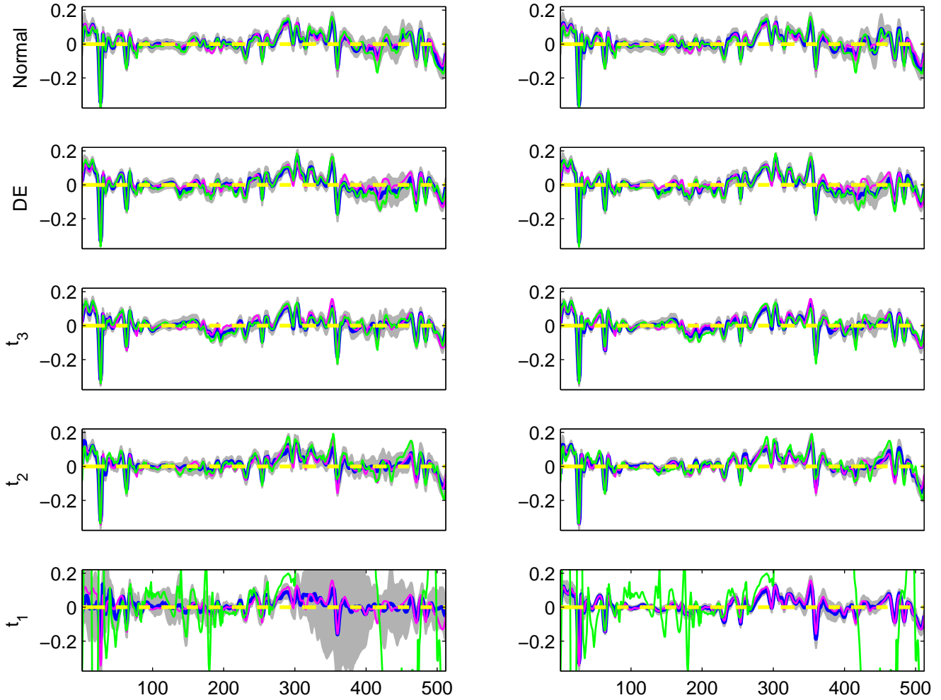
The estimated B_5(t) for 5 simulated datasets, simulation run 2 G-WFMM R-WFMM
