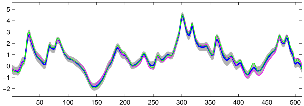
Estimated C_0(t) using R-WFMM: Normal data, run 2
