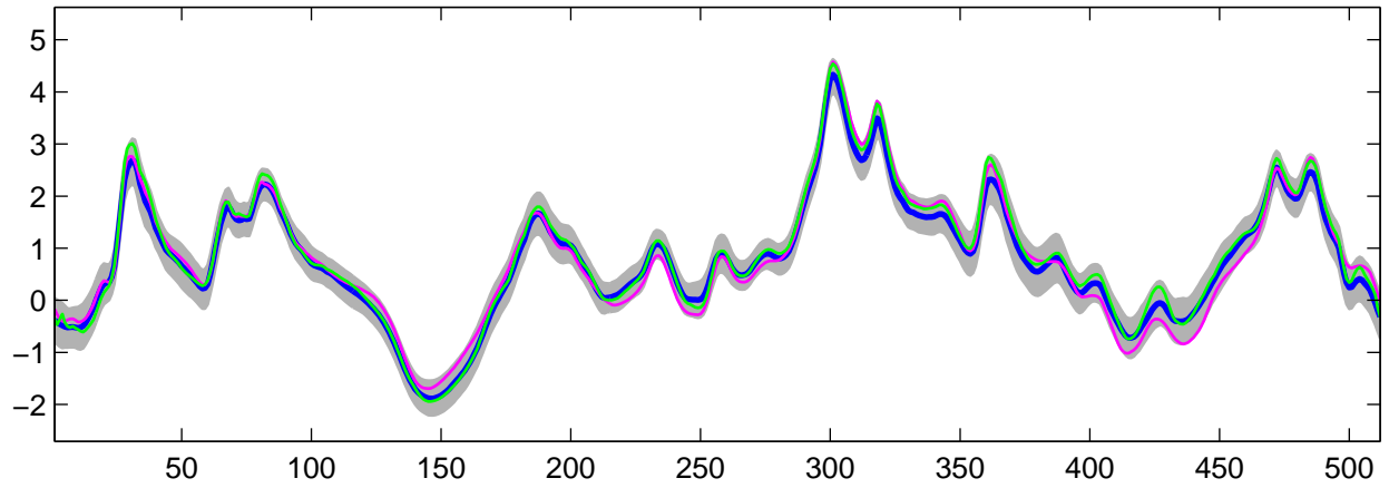
Estimated C_0(t) using G-WFMM: Normal data, run 2
