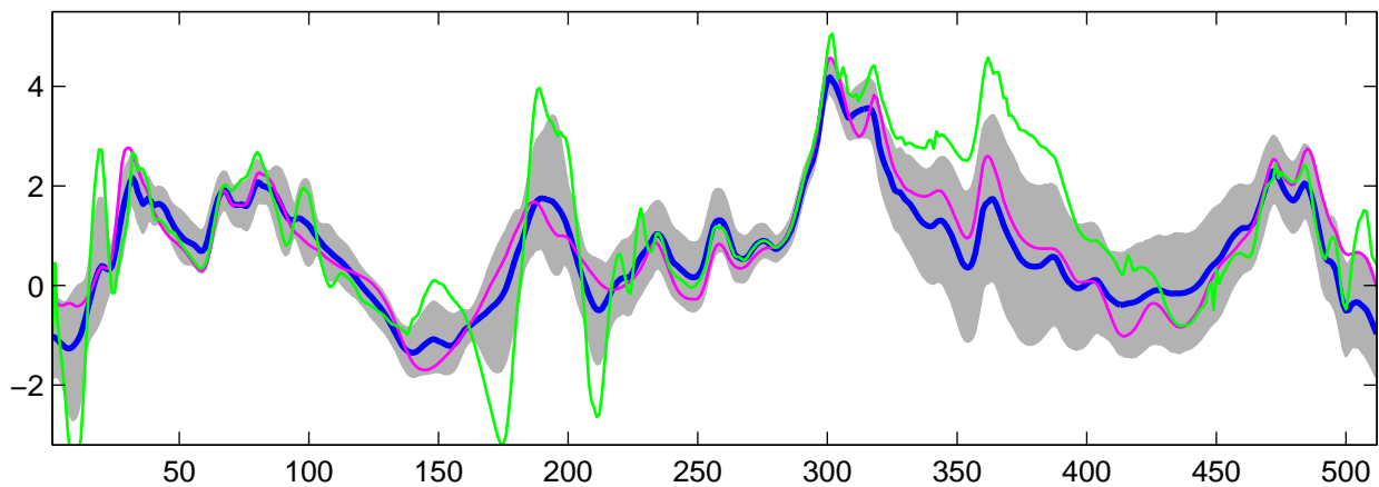
Estimated C_0(t) using G-WFMM: t_1 data, run 2
