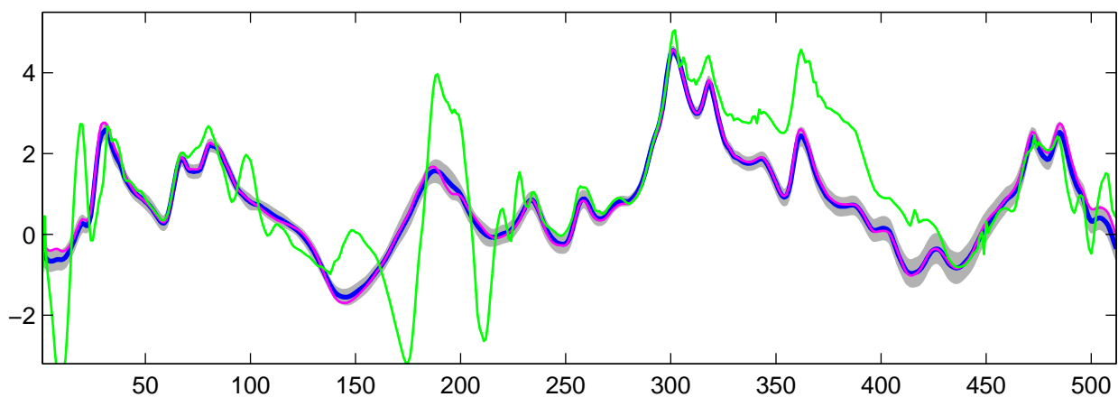
Estimated C_0(t) using R-WFMM: t_1 data, run 2
