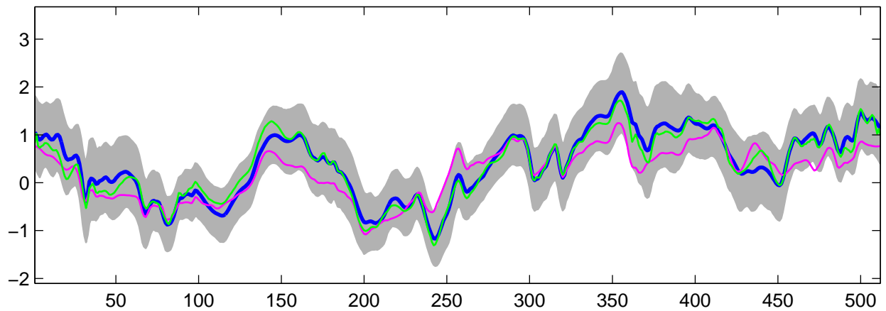
Estimated C_1(t) using R-WFMM: Normal data, run 2
