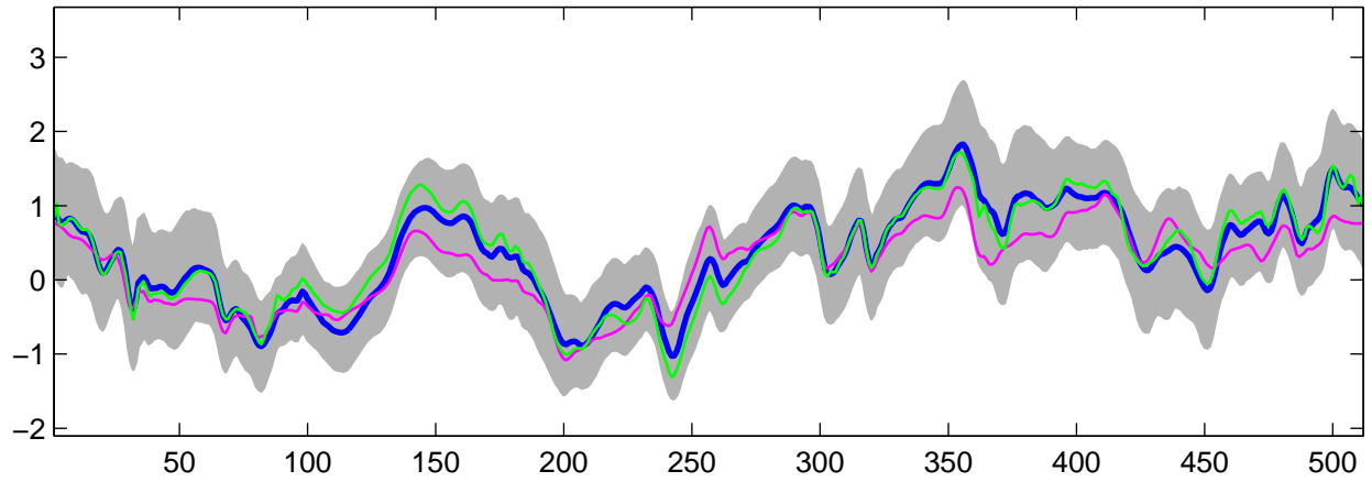
Estimated C_1(t) using G-WFMM: Normal data, run 2
